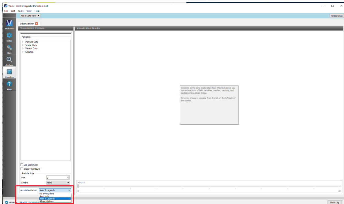
Fig. 11.3: Annotation Level
