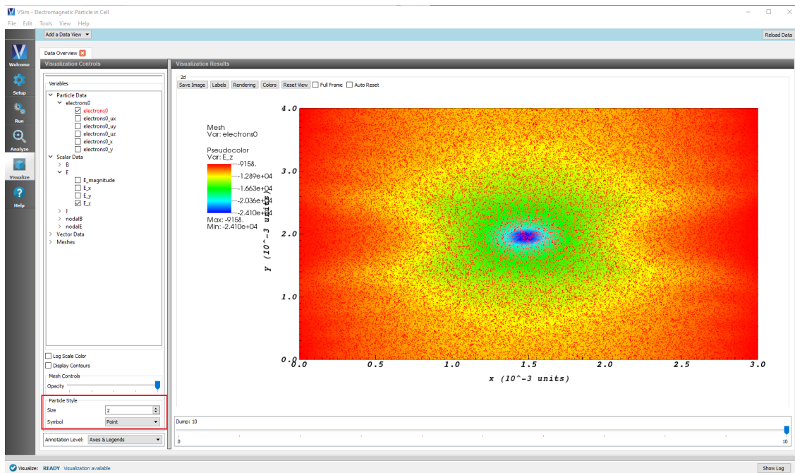
Fig. 11.14: Particle Style
