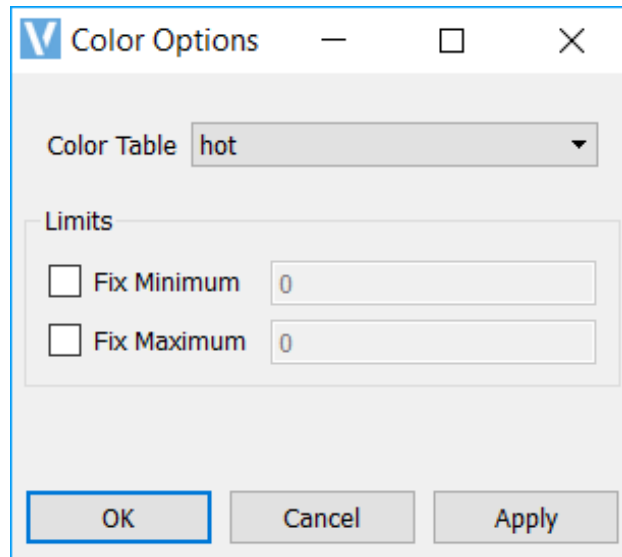
Fig. 11.8: Colors Menu
