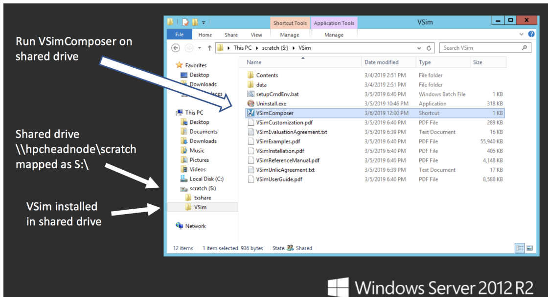
Fig. 8.11: VSIm must be installed in the shared drive to run Vorpai on a Windows Cluster.
