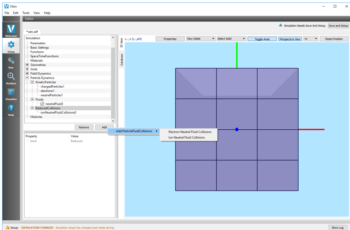
Fig. 6.18: Collisions
