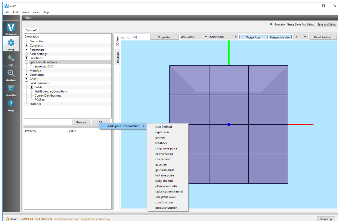
Fig. 6.6: SpaceTimeFunctions definitions
