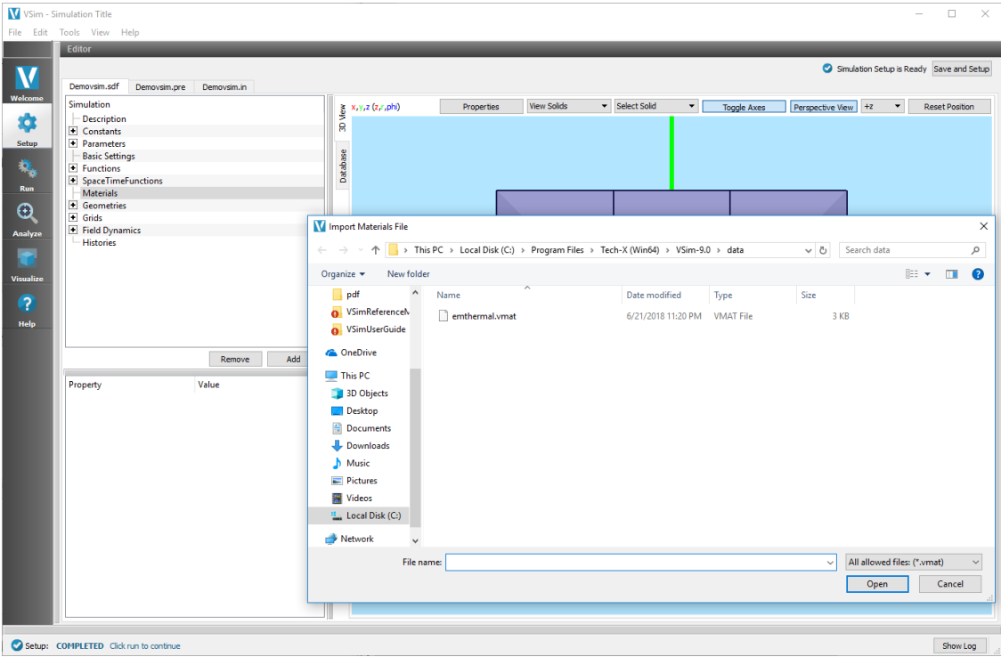
Fig. 6.7: Importing materials
