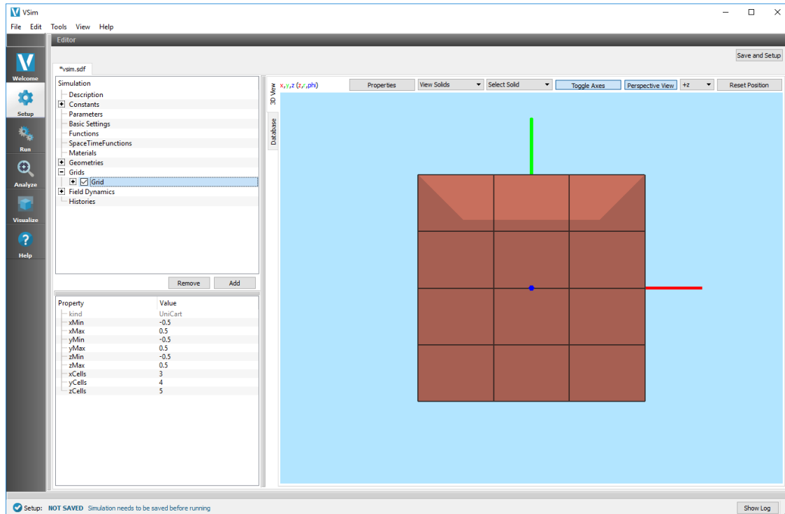
Fig. 6.14: Grid settings
