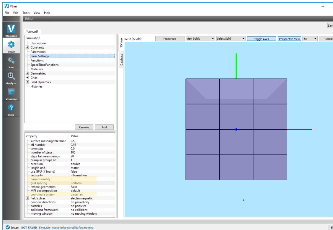
Fig. 6.13: Grid choices
