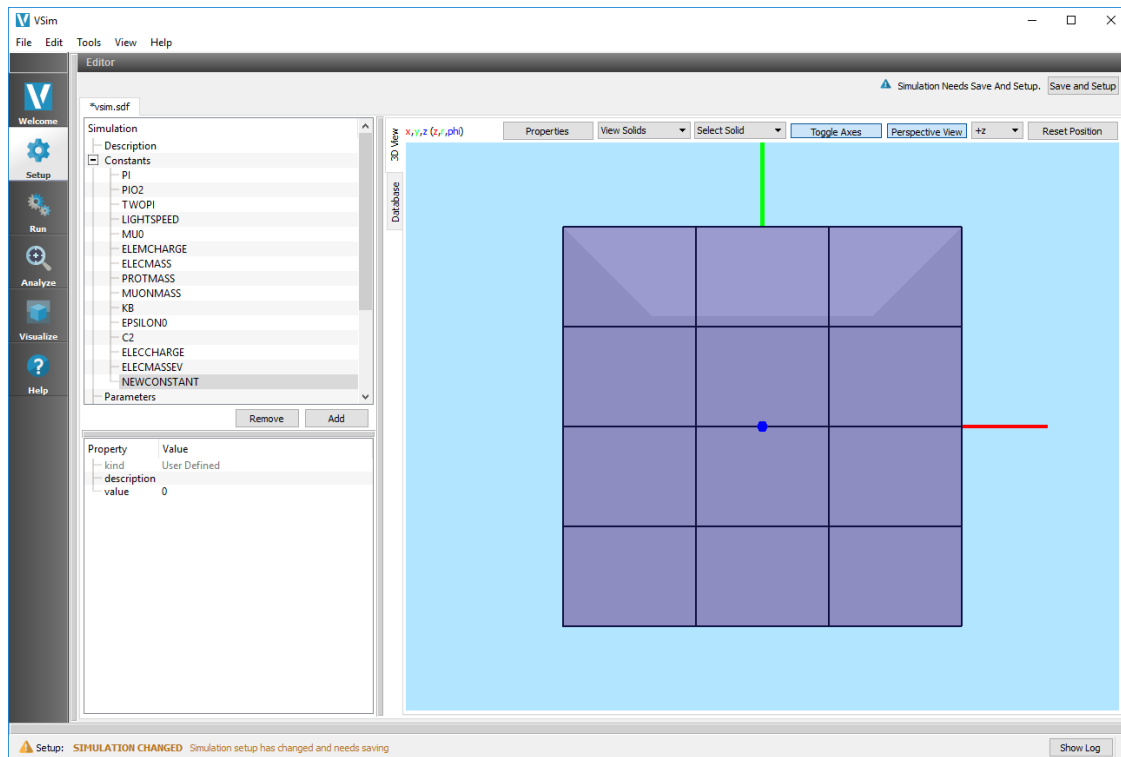
Fig. 6.3: Constant definitions
